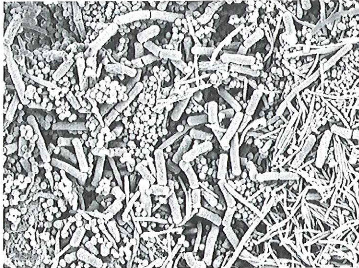
Figure 1. Scanning electron micrograph of biofilm grown from the subgingival plaque of a healthy subject for 10 days anaerobically on saliva-coated hydroxyapatite discs. (Grown by Michael Sedlacek, PhD, and Clay Walker, PhD, at the University of Florida College of Dentistry Periodontal Disease Research Center. Image taken by the University of Florida Electron Microscopy Core Facility.)
